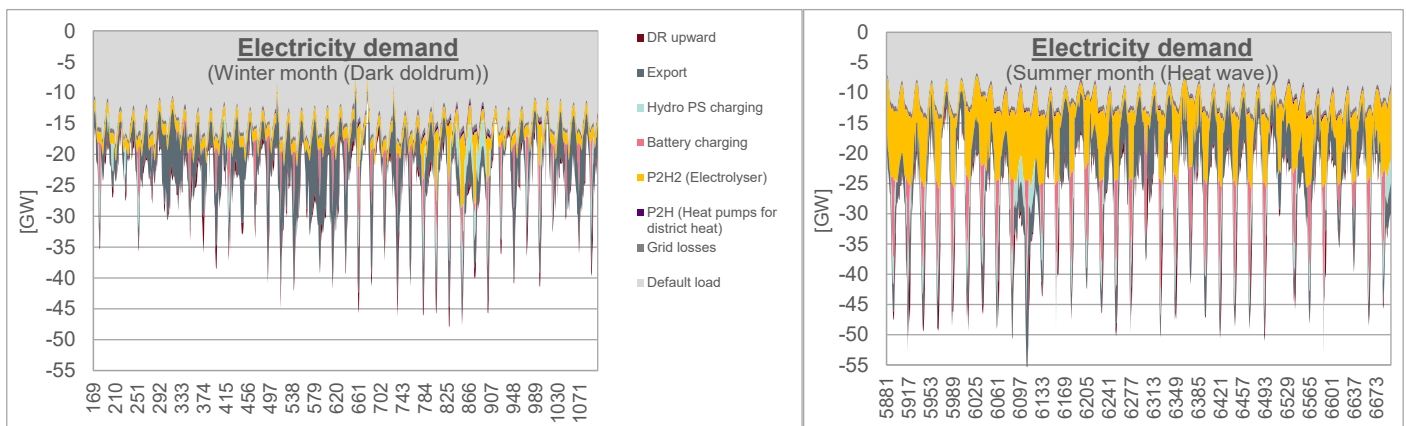
Figure 11: Electricity supply and demand in Austria by 2050 according to the DN pathway for a dark doldrum during winter (left) and a heat wave during summer (right)
