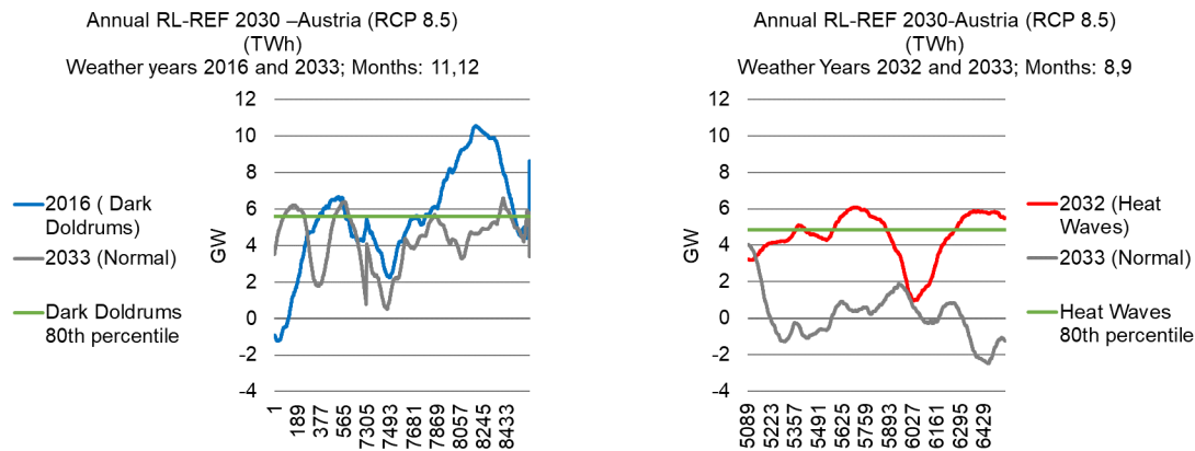
Figure 22: Representation of Peak Periods of Residual Load (PPRL) in the case of REF-2030 by considering RCP 8.5
