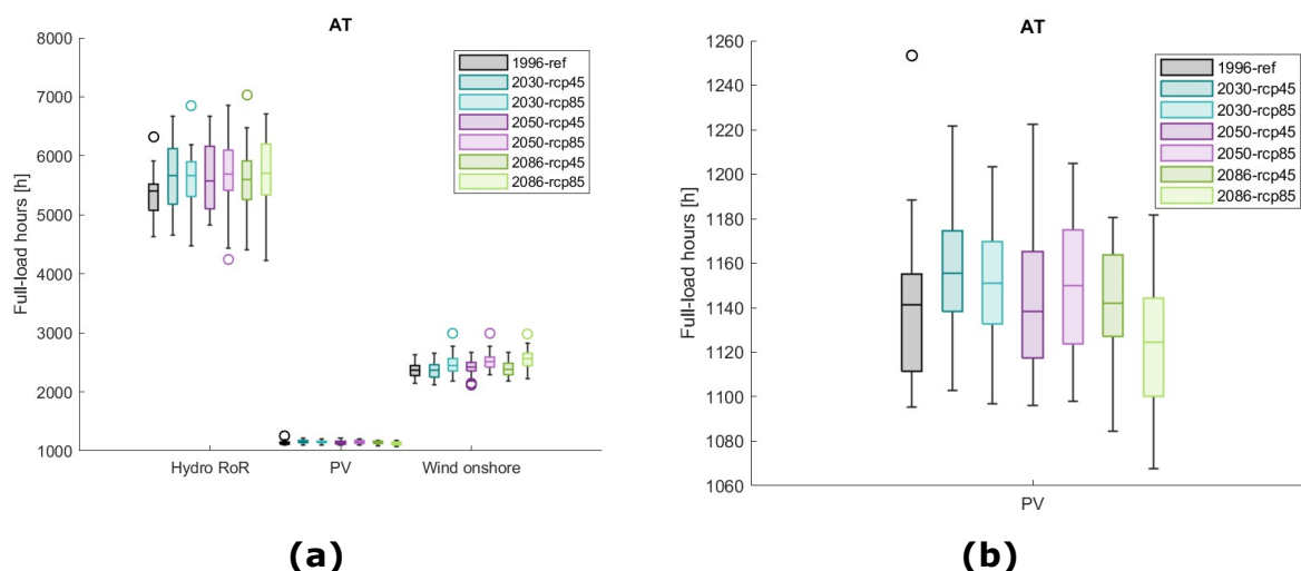
Figure 4: Development of full-load hours of run-of-river (RoR) hydropower, PV, and wind onshore (Panel (a)) and PV in greater detail (Panel (b)) in Austria in the two considered climate scenarios (rcp4.5 and rcp8.5) compared to the reference period (1981-2010); each box represents 30 weather years around the target year; the reference period is based on ERA5-Land.
